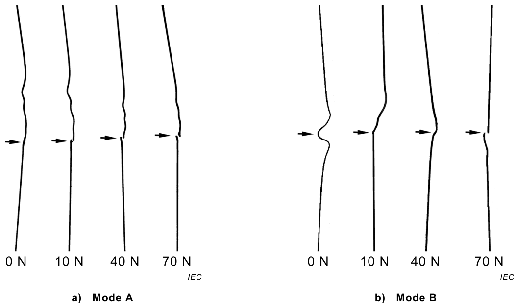
Figure B.3 – Side views of the specimens after failure with Mode A and Mode B for different tensile forces
